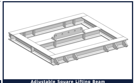
Adjustable Square Lifting Beam
